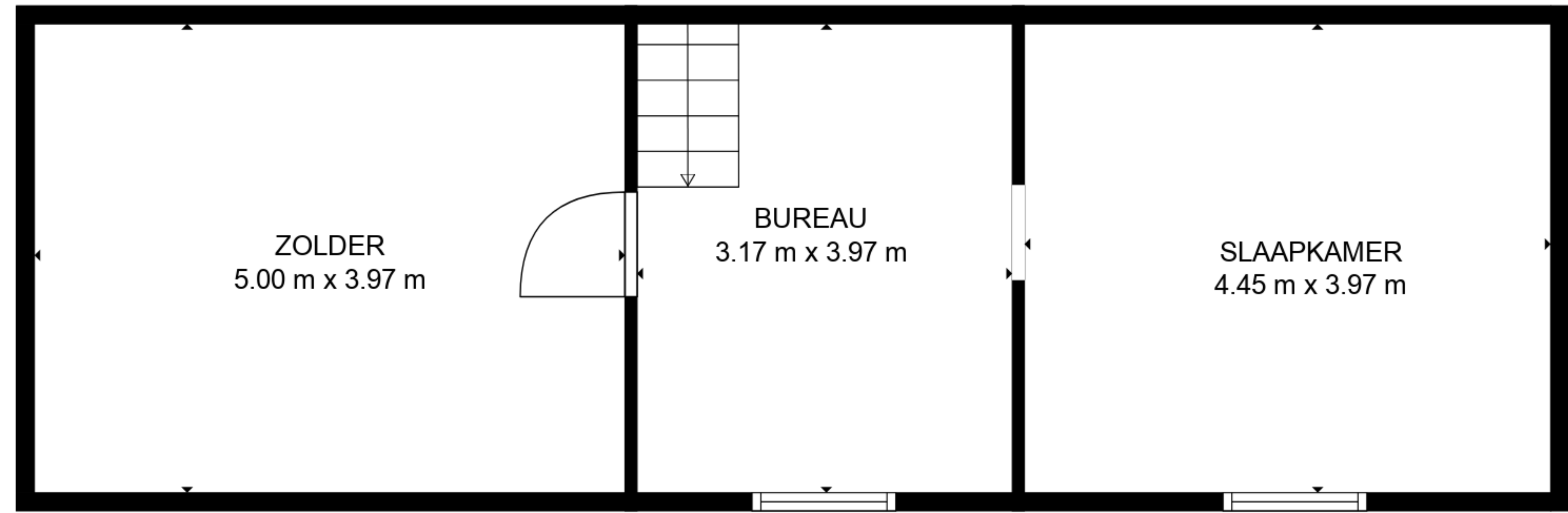
3. ZOLDER
